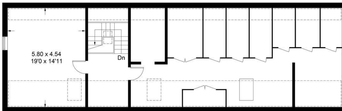
First Floor
